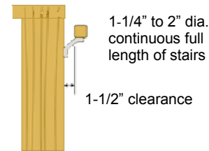
Handrail cross-section
